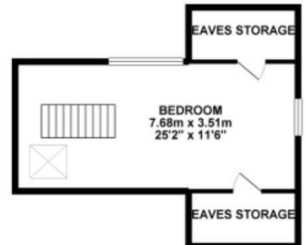
2ND FLOOR 35.70 sq. m. ( 384.23 sq. ft. )
