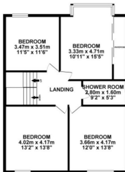
1ST FLOOR 77.19 sq. m. ( 830.91 sq. ft. )
